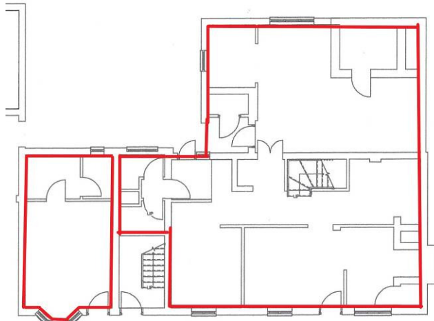
0 - Existing Ground Floor 1:50
